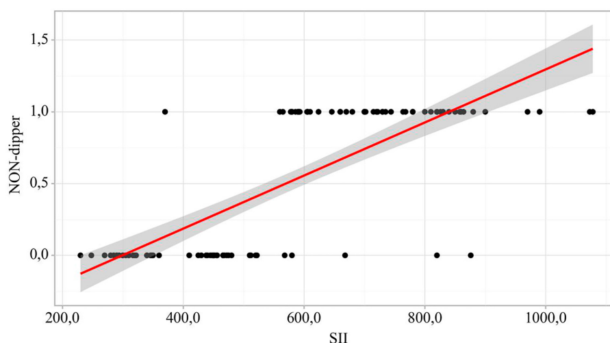
Fig. 1. Regression function graph characterizing the «non-dipper» dependence upon SII.
